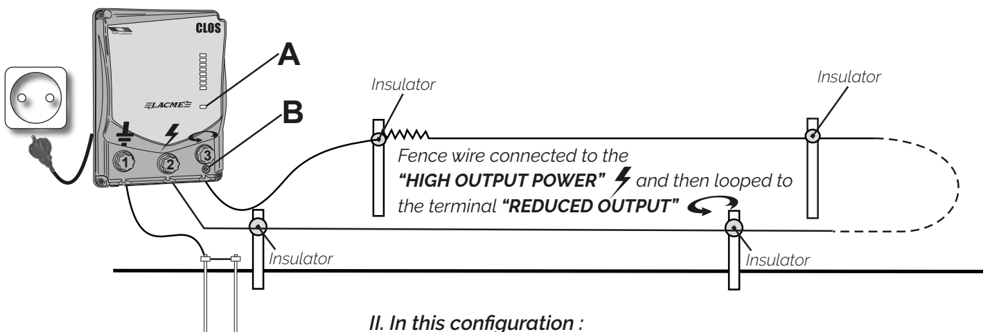
Example of a loop connection :
